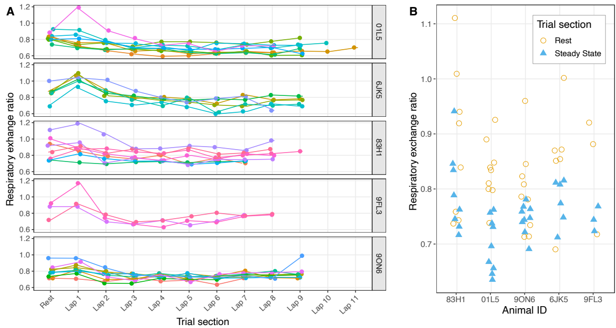
Fig. S1. Respiratory exchange ratio (RER; V_{CO_2} V_{O_2}^{-1} ). RER for five dolphins during 35 trials. A) Mean RER per rest or per lap; each line represents one trial. B) Points represent mean RER during rest or during steady-state periods.
