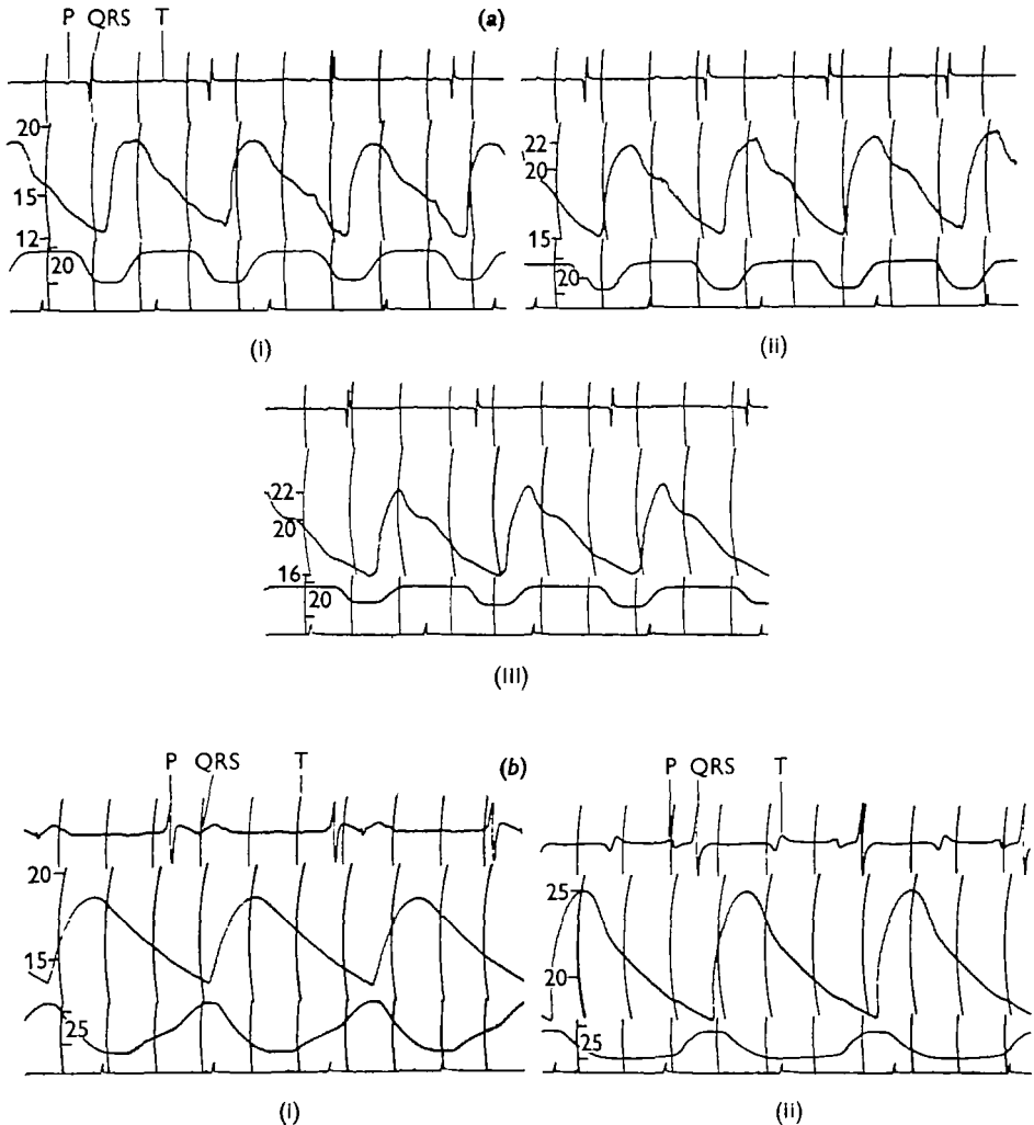
Fig. 7. Ventricular volume and systemic blood pressure in: (a) R. pipiens (21 g.)—(i) at surface, (ii) submerged 6 min., (iii) submerged 11 min.; (b) R. temporaria (31 g.)—(i) and (ii) at surface, 90 min. apart. Trace 1, electrocardiogram; trace 2 systemic blood pressure (mm. Hg); trace 3, ventricular volume ( \mu l.), in (a) up on trace = decrease in volume, in (b) down on trace = decrease in volume; trace 4, time (sec.). Curved lines show writing radius of pens and coincident points in time.
