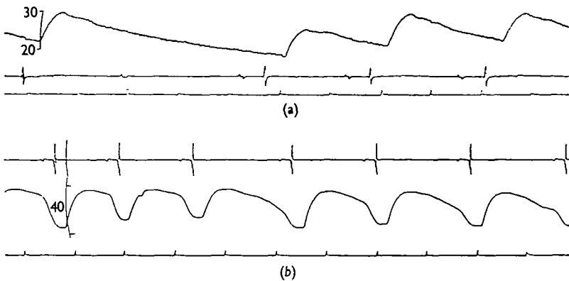
Fig. 5. The effect of arrhythmic heart beat. (a) Pulmocutaneous pressure. R. pipiens (23 g.). Trace 1, pressure (mm. Hg); trace 2, electrocardiogram; trace 3, time (sec.). (b) Stroke volume. R. pipiens (21 g.). Trace 1, electrocardiogram; trace 2, volume ( \mu l., up on trace = decrease in volume); trace 3, time (sec.).
