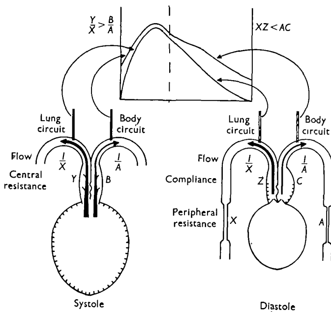
Fig. 11. Diagram to show relationships between resistance, compliance and flow in the body and lung circuits which will result in the characteristic pulse curves. For further explanation see text.
