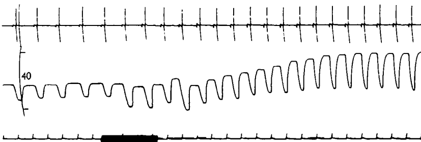
Fig. 9. The effect of surfacing on the total and stroke volume of the ventricle of R. pipiens (21 g.). Trace 1, electrocardiogram; trace 2, stroke volume ((μl.), up on trace = decrease in volume); trace 3, time (sec.), mark indicates emersion.
