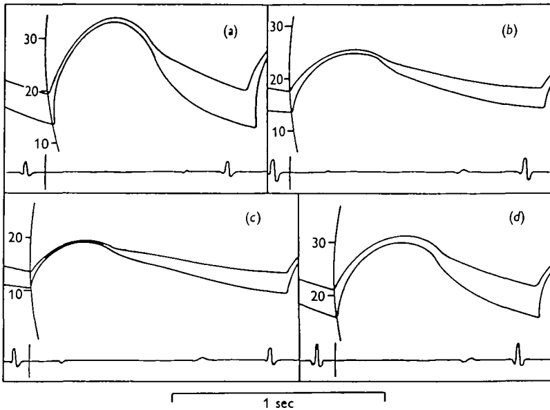
Fig. 6. Pressures (mm. Hg) recorded from systemic and pulmocutaneous arches in R. temporaria (32 g.) and superimposed as explained in text. The systemic pressure is the top trace in all cases. The calibration curve and the corresponding curve on the e.c.g. trace show the writing radius of the pens and represent the same point in time: (a) at surface; (b) submerged 11 min.; (c) submerged 22 min.; (d) surfaced 10 min.
