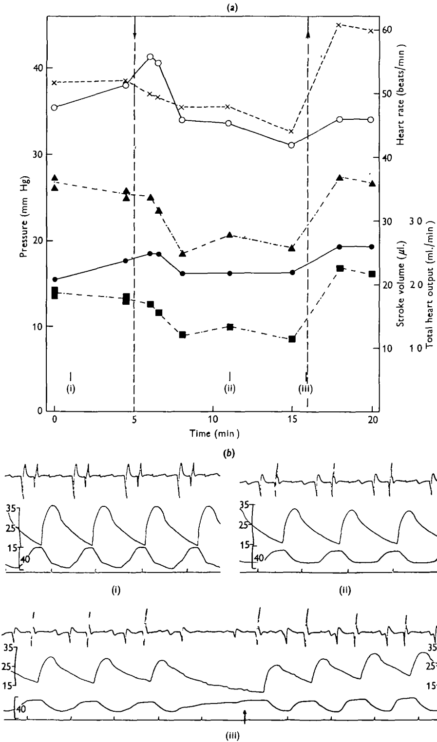
Fig. 10. (a) Heart output, carotid blood pressure and heart rate in R. temporaria (35 g.). Downward and upward pointing arrows indicate submersion and emersion respectively. \times , Heart rate, O , systolic pressure; \bullet , diastolic pressure; \blacktriangle , stroke volume; \blacksquare , minute volume. (b) Pressure pulses (mm. Hg) and stroke volumes ( \mu l.), down on trace = decrease in volume) recorded at times indicated on graph.
