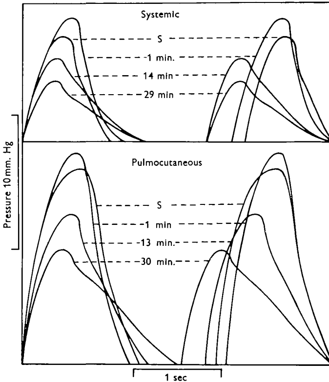
Fig. 3. Pulses recorded from systemic and pulmocutaneous arches in R. pipiens at the surface and after the periods of submersion indicated. The same pulses are superimposed using the beginning and end of the pulse wave as the point of coincidence.
