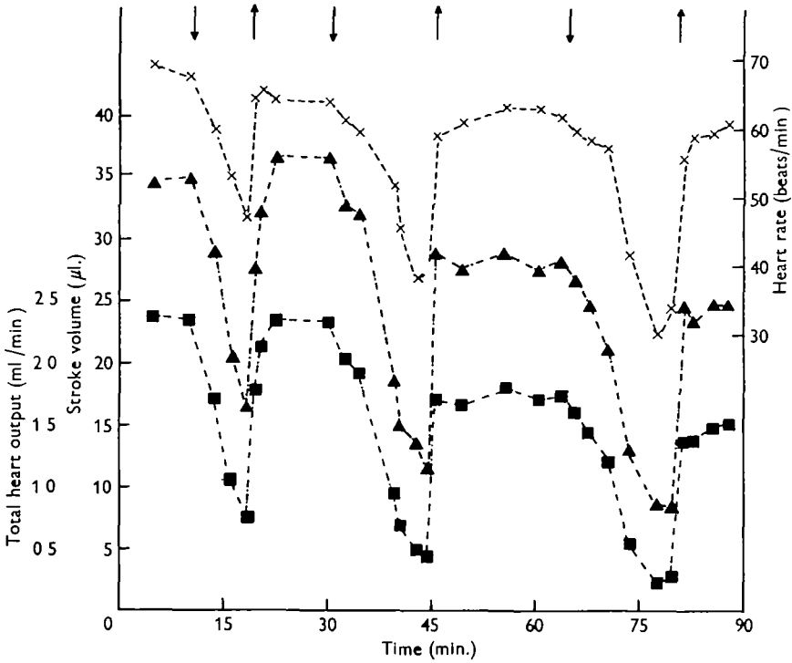
Fig. 8. Stroke volume, minute volume, and heart rate in R. pipiens (21 g.). Downward and upward pointing arrows indicate submersion and emersion respectively. ×, Heart rate; ▲, stroke volume; ■, minute volume.
