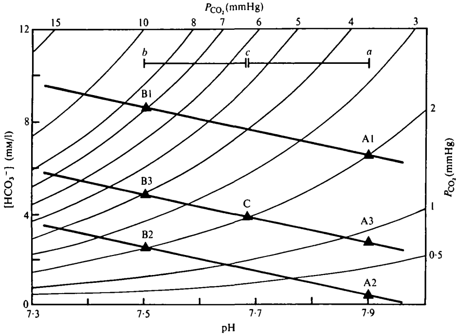
Fig. 1. Davenport diagram for flounder blood relating [\text{HCO}_3^-] , pH, and P_{\text{CO}_2} (isopleths in mmHg). Parallel lines A_1 B_1 , A_2 B_2 , and A_3 B_3 represent buffer lines of slope \beta as determined in vitro . The figure illustrates the method employed in determining the fraction of a total pH drop (horizontal distance ab ) which would have been due to lactic acid changes alone ( ac/ab ) and the additional fraction due to P_{\text{CO}_2} changes ( bc/ab ). A_1 = initial point at rest. A_1 B_1 : pH drop is due solely to P_{\text{CO}_2} increase. A_2 B_2 : pH drop is due solely to lactic acid increase. A_3 B_3 : pH drop is due to both factors. See text for further details.
