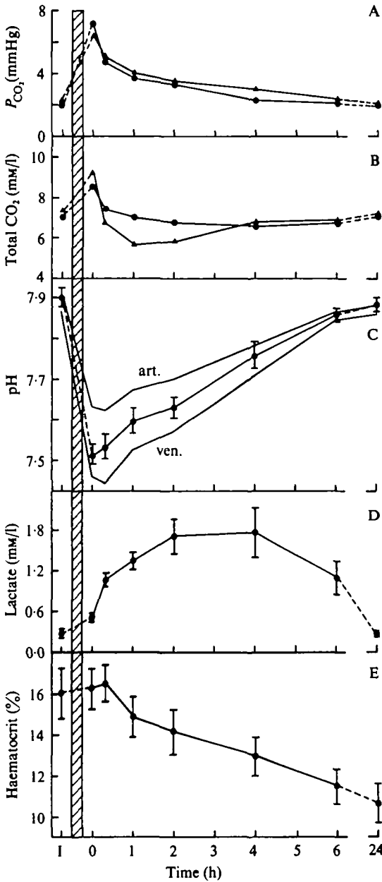
Fig. 3. (A) P_{CO_2} (as calculated by the Henderson-Hasselbalch equation) and (B) total CO_2 concentration in the venous blood of two flounders ( \bullet = 800 g, \blacktriangle = 450 g); average (C) pH, (D) lactate concentration, and (E) haematocrit in the venous blood of six flounders (means \pm 1 s.e.) before and after 10 min of exhausting activity. In (C) simultaneous measurements of arterial and venous pH in a single flounder (330 g) are indicated by plain lines. Activity = bar. I = initial resting sample. Time 0 = immediately post-exercise.
