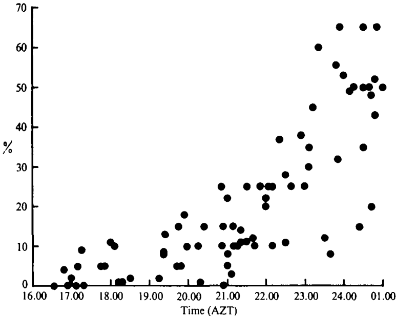
Fig. 3. The extensibility of Manduca wings tested at different times during the hours preceding adult eclosion. The ordinate shows the percentage extension of the wings 3 min after loading. The normal 'gate' for eclosion is from 23.00 AZT onward.
